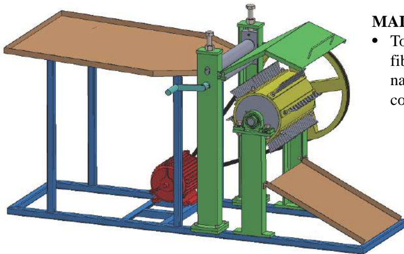
HACKLE (CAD MODELING)
