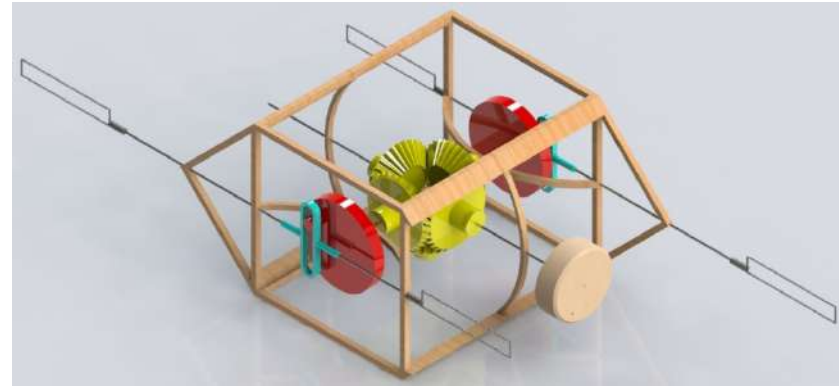
MULTIPURPOSE MACHINE (SAW AND GRIND) USING SCOTCH YOKE MECHANISM
